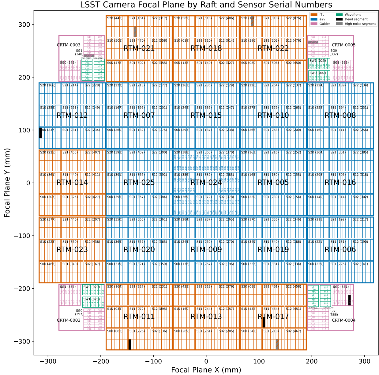
FIGURE 2: Focal plane layout including raft and CCD serial numbers (see text). The raft and CCD serial numbers come from the eTraveler database accessed using datacat-utilities ( https://github.com/lsst-camera-dh/datacat-utilities ). The bad segment list is as in 1.
